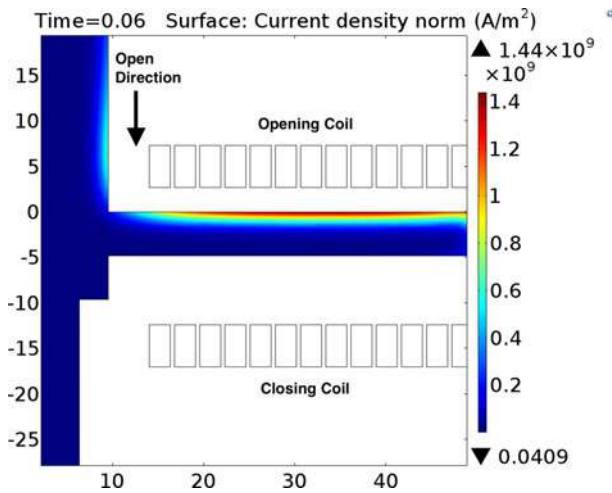
Fig. 9. Induced current in the disc, 60 \mu s after energizing the opening coil, simulation in axisymmetric 2-D view.
