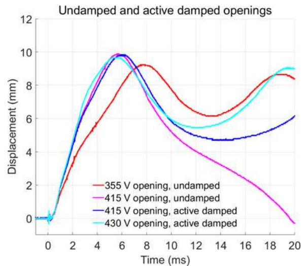
Fig. 11. Damped and undamped operations.
