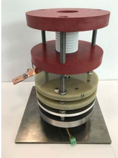
Fig. 4. UFMS prototype. (Base plate is approximately 30 cm \times 30 cm.)
